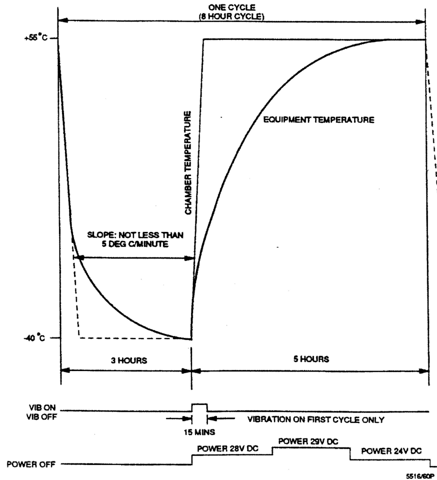
Figure 2-3 - The Burn-In Thermal Cycle
