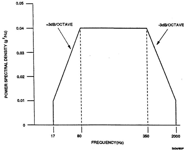
Figure 2-2 - Random Vibration Spectrum
